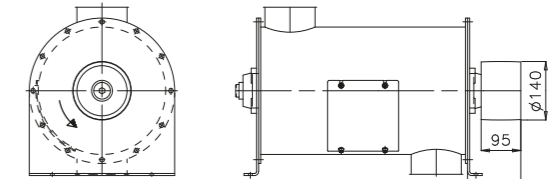
VERSION WITH ROUNDED PULLEY FOR FLAT BELT
