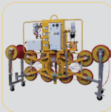
Optional Kombi wheeled trolley
