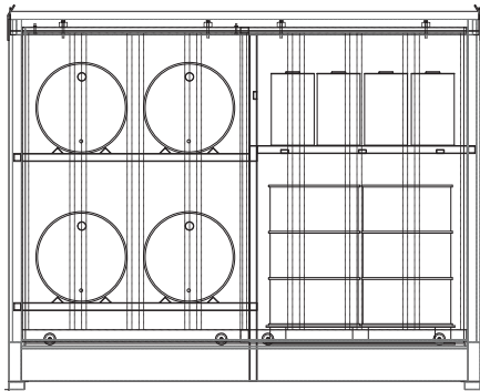
STORAGE LAYOUT IN A DS12S
