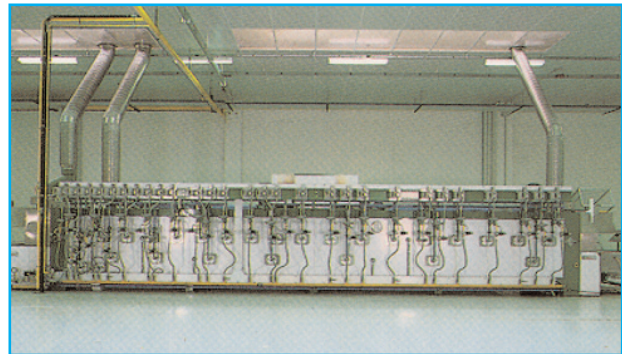
Pizza baking oven with direct flame burners, model Ribbon (Simer)
