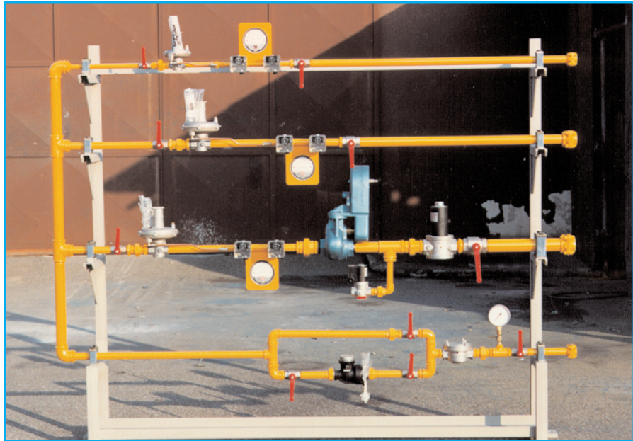
Gas decompressing systems for 3-area combustion plants (Continuous)
