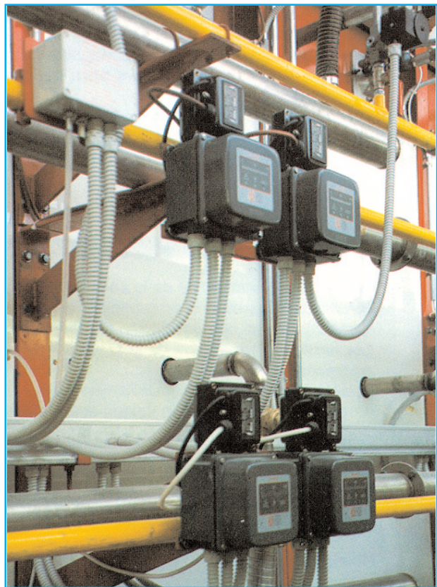
Sanitary fittings baking furnace with "Nozzle Mix" burners (Intercer)
