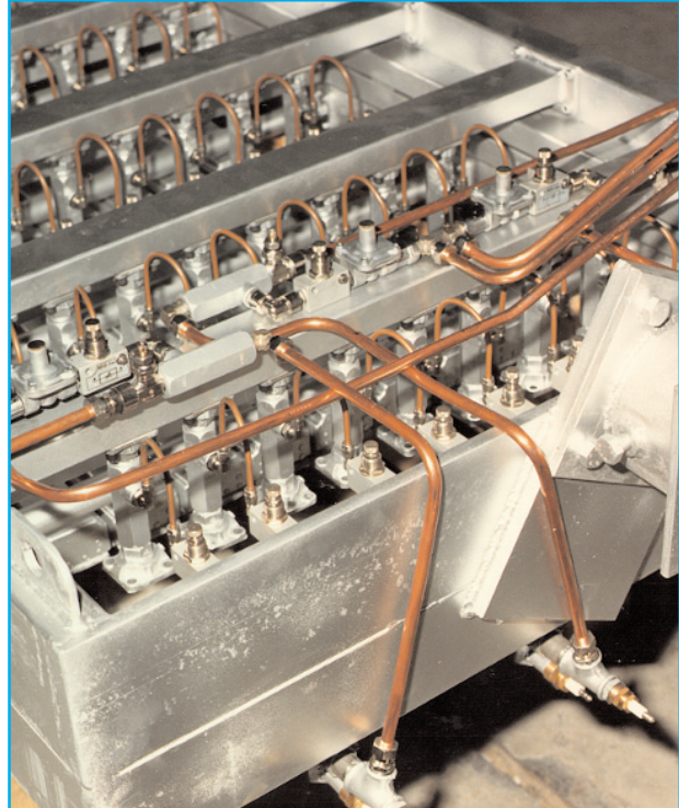
Manifold with metallic, infrared burners, model BR-70/300, for paper drying (Cartiera Nicoli)
