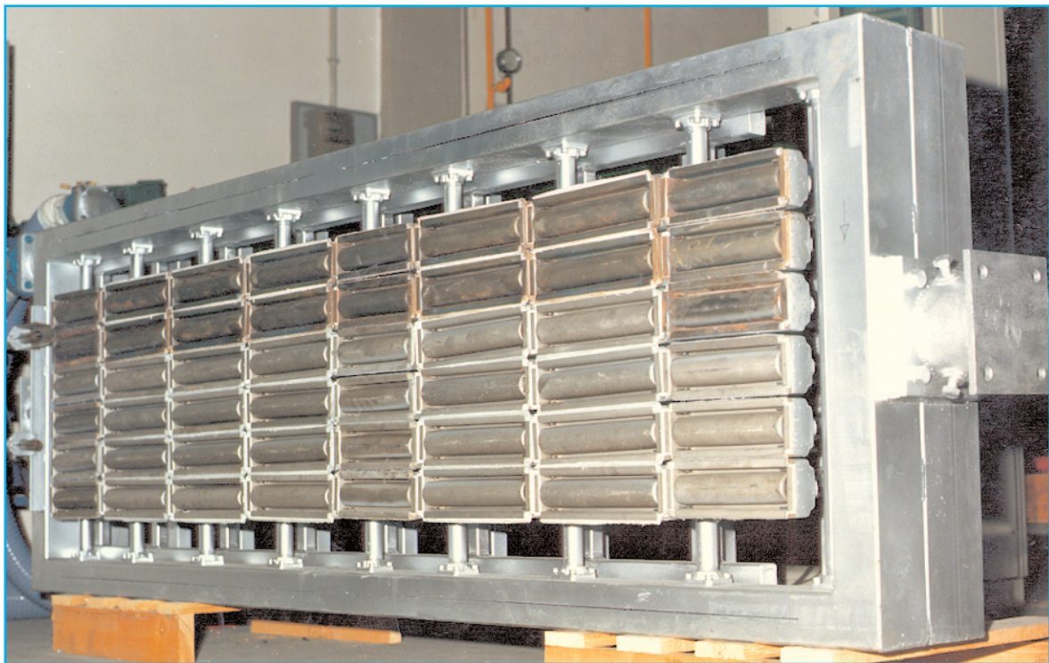
Manifold with metallic, infrared burners, model BR-70/300, for paper drying (Cartiera Nicoli)
