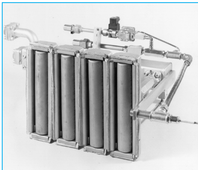
Radiant panel with infrared burners, model BR-70/300 (Murrina d'arte)
