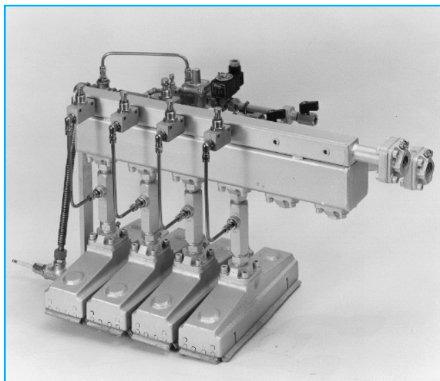
Radiant panel with infrared burners, model BR-70/300 (Guido Farinati)
