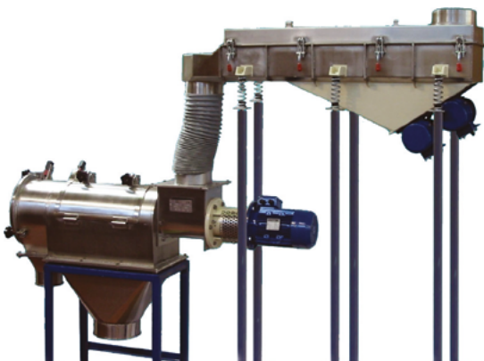
- Screening/refining unit
