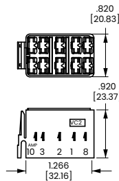
VC2 CONNECTOR HOUSING (For AMP terminals only)
