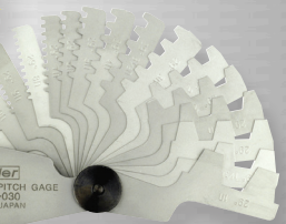
Acme Screw Pitch Gage 52-485-030-0
