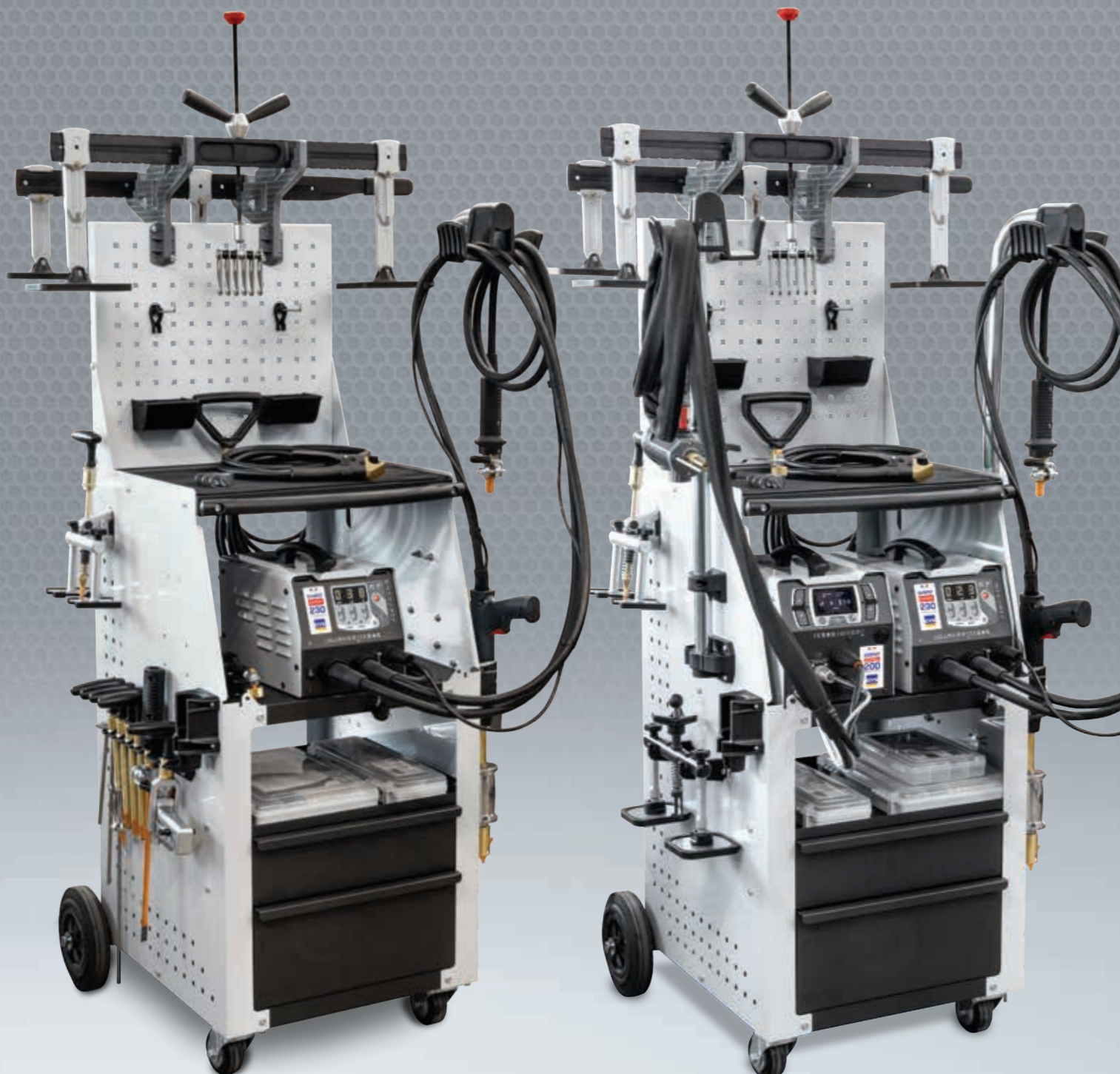
ARCPULL 200 + PRO 230, 400
