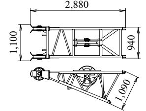
Jib Upper Spreader (for Luffing) Weight: 260 kg
