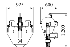
70 t Hook Weight: 1,200 kg
